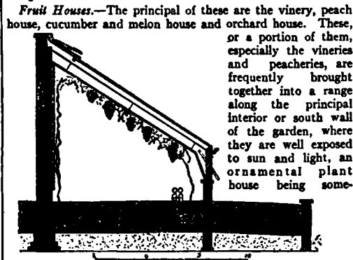
FIG. 5.—Lean-to Vinery.
