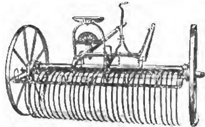
FIG. 4.—Self-acting Horse Rake. (Ransomes, Sims & Jefferies, Ltd.).
