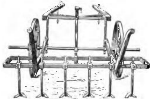
FIG. 3.—Martin's General Purpose Steerage Horse Hoe.
