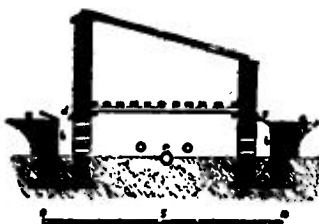
FIG. 10.—Ventilated Plant Pit.
