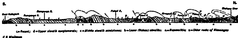
Section across the sub-Himalayan zone.
