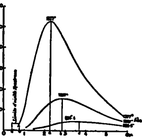
FIG. 7.—Distribution of energy in the spectrum of a black body.
