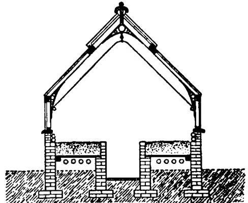
FIG. 9.—Forcing House.
