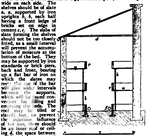
FIG. 13.—Lean-to Mushroom House.
