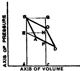
FIG. 5.—Elementary Carnot Cycle for Gas.
